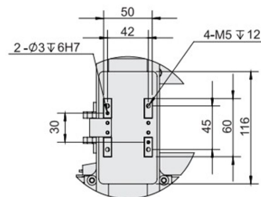
B-Detail View
