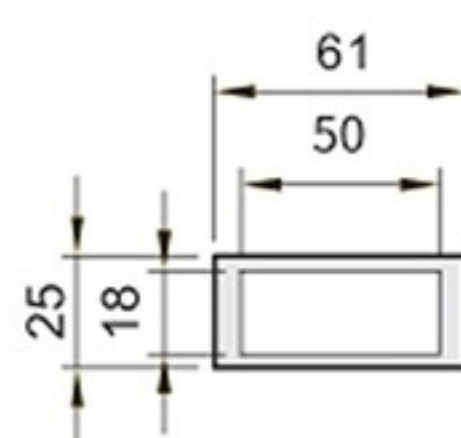
XY-Cable Chain
