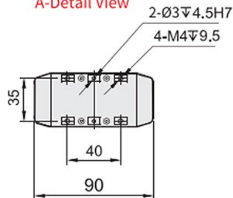
A-Detail View
