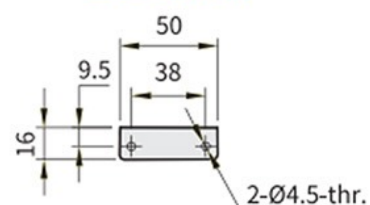
C-Detail View
