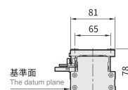
C-C View
