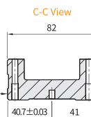
C-C View
