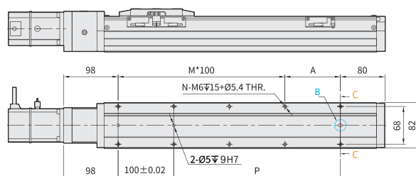
B View
